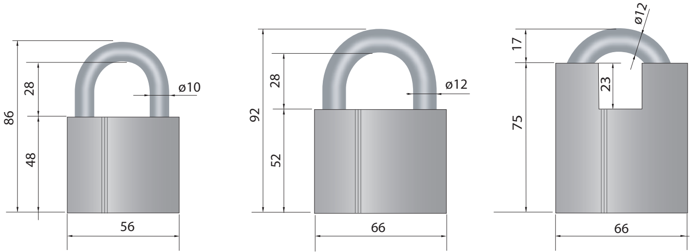
HSS Padlock Dimensional Drawing
