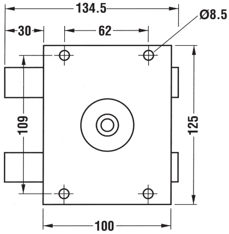
G2000 Dimensional Drawing
