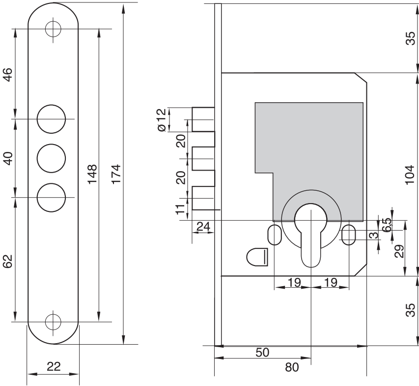
ZW 550 RYS Dimensional Drawing
