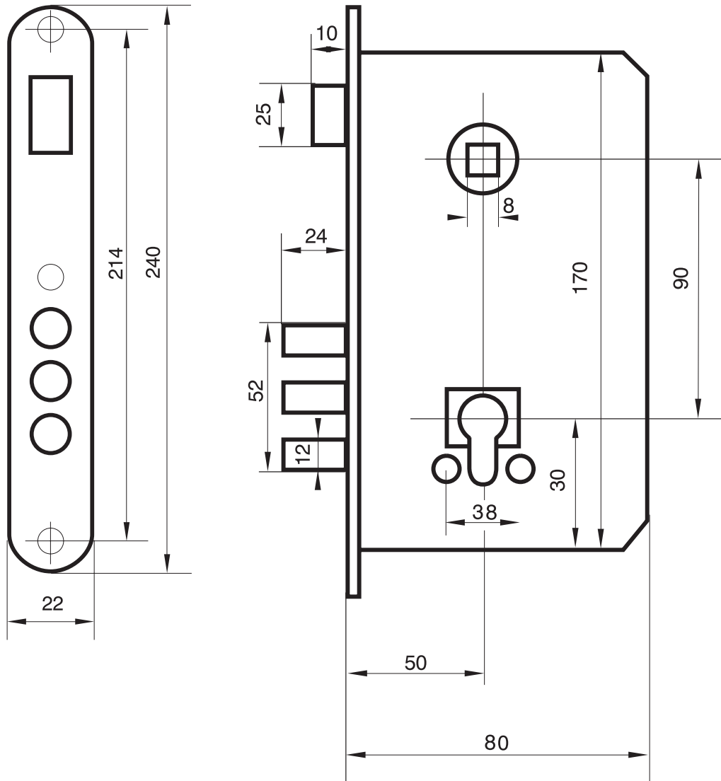
ZW1000 Dimensional Drawing Width of ZW1000 lock = 17mm
