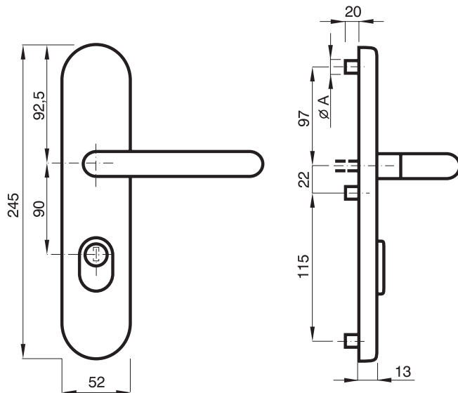
TD200 Outside Dimensional Drawing
