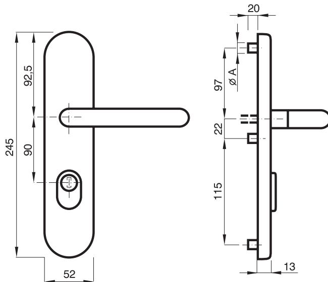
TD1000 and TD2000 Outside Dimensional Drawing
