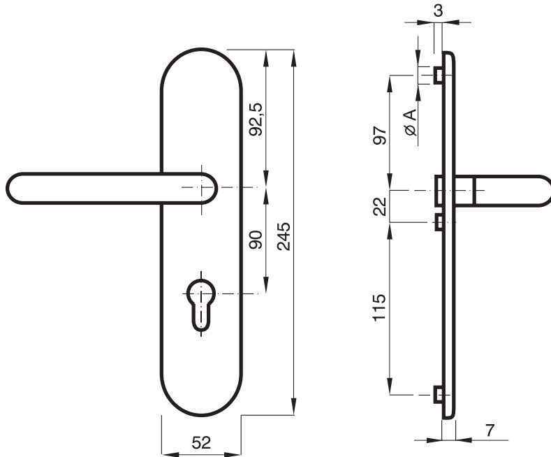
TD1000 and TD2000 Inside Dimensional Drawing
