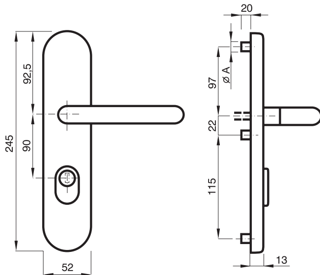
TD1000 Outside Dimensional Drawing
