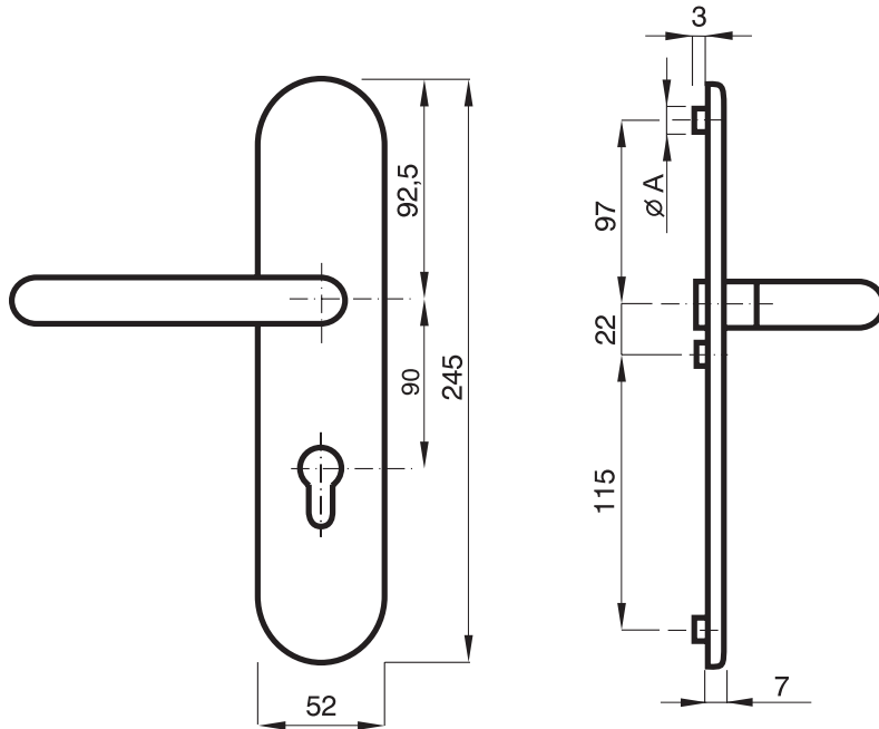
TD1000 Inside Dimensional Drawing
