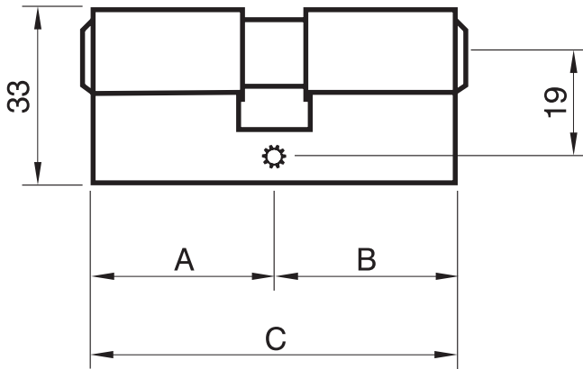
M3 Dimensional Drawing
