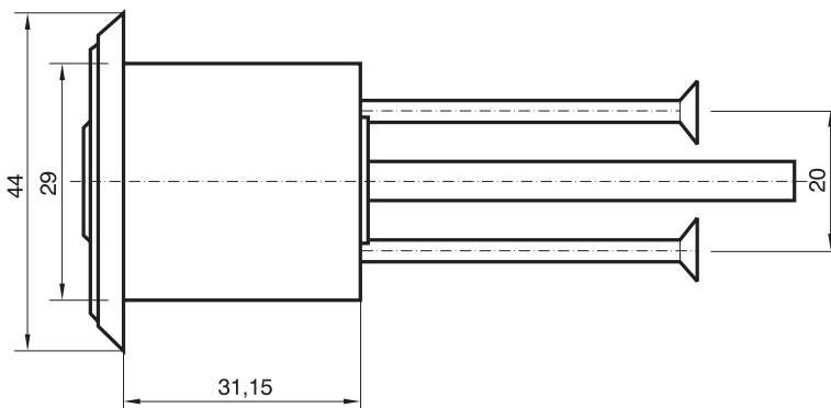
M3Z Dimensional Drawing
