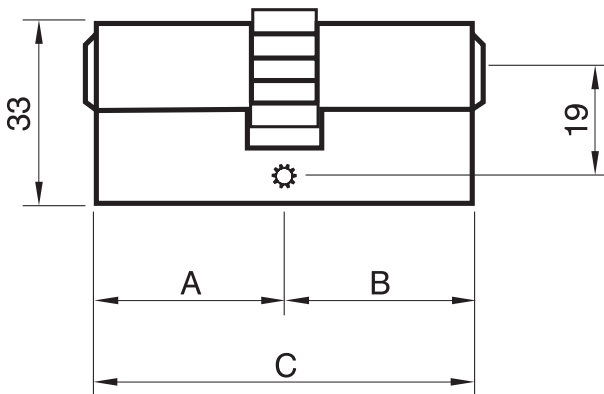
M3Z Dimensional Drawing
